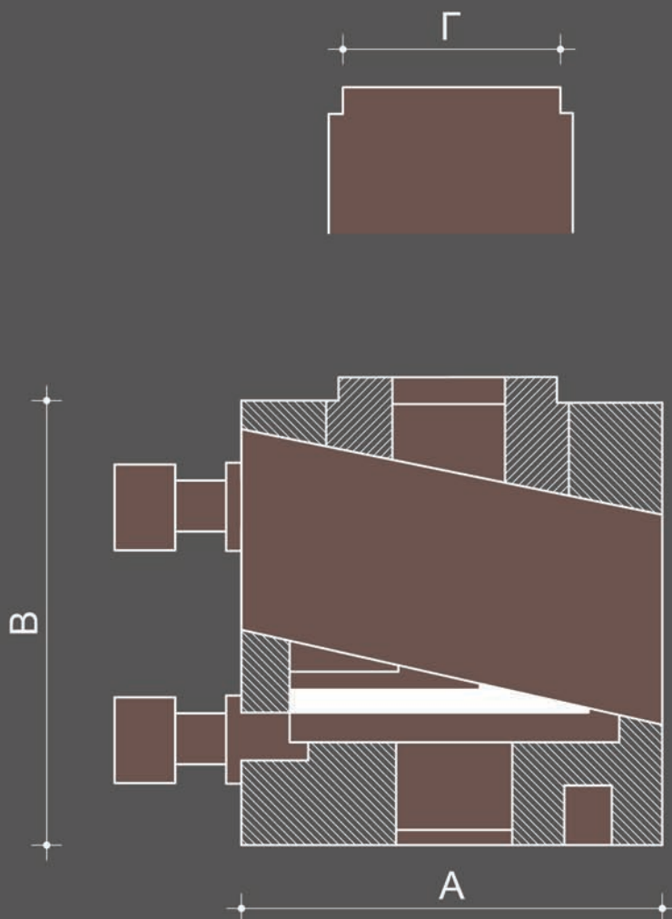
DOUBLE ACTING HOLLOW PLUNGER CYLINDERS 20Ton TO150Ton
